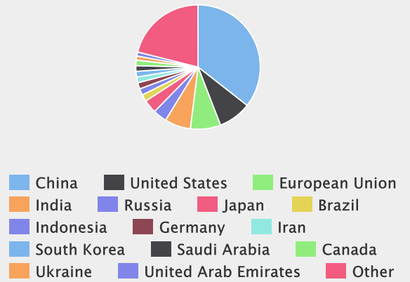
Industry > CO2 emissions from manufacturing industries and construction > Million metric tons, 2011
