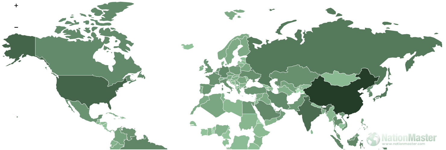
Industry > CO2 emissions from manufacturing industries and construction > Million metric tons, 2011
